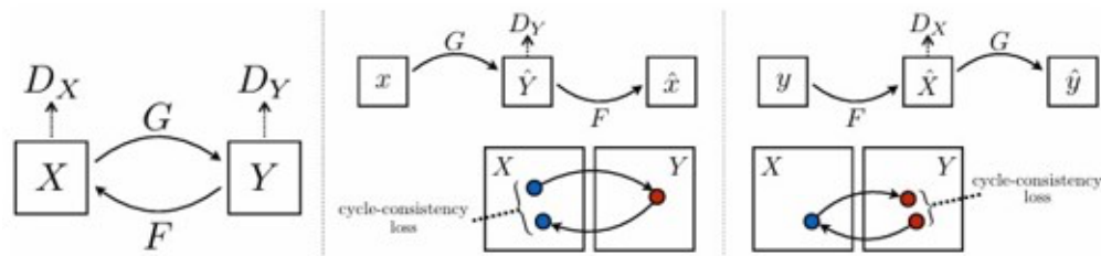
Figure 1 Concept CycleGAN
